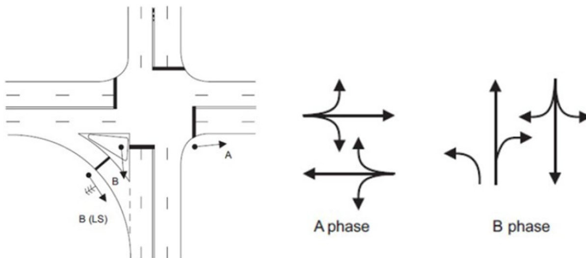
Figure 10.4 – Late start for large corner islands
