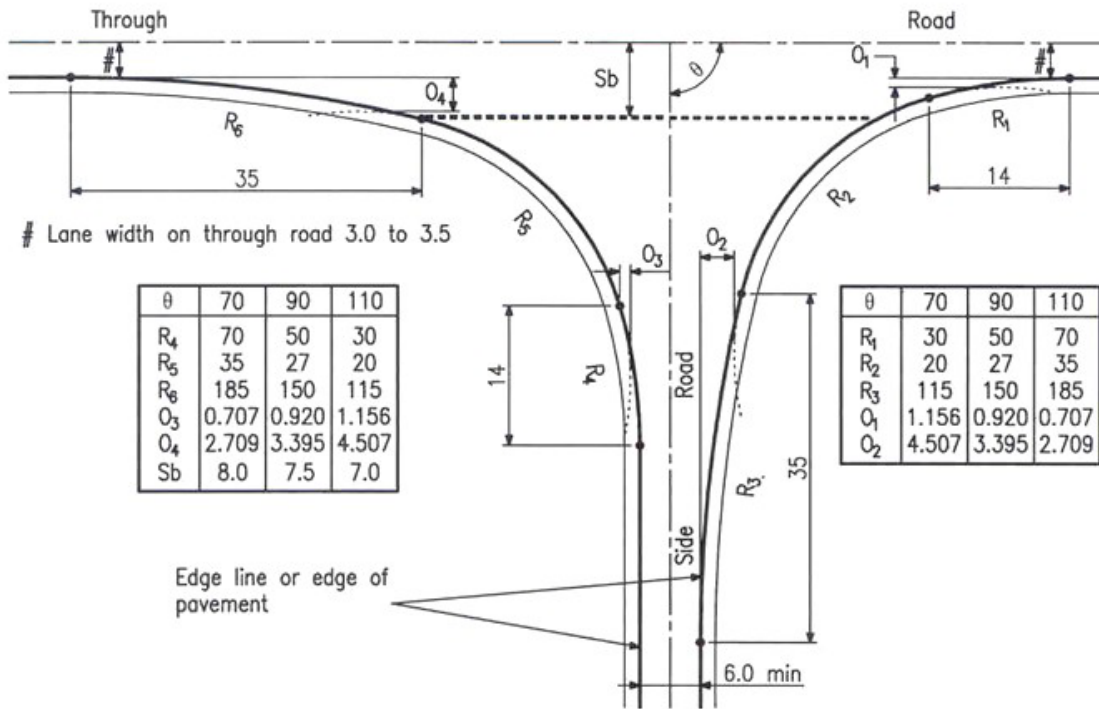
Figure D(c) – Details of type 'BAL' layout for rural sites to suit type 2 (triple) road train operation
