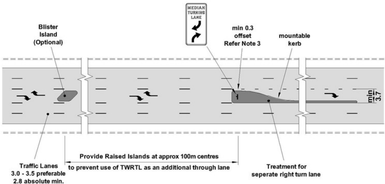
Figure 4.4 – Two-way right-turn lanes on an urban road
