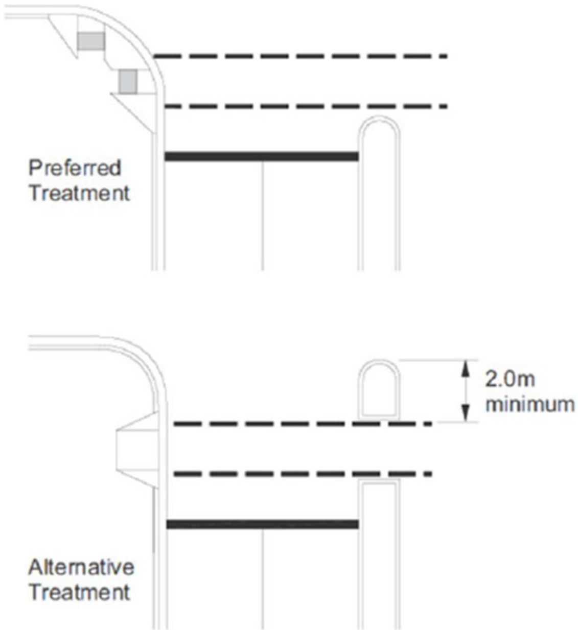
Figure 10.7(b) - Treatment of pedestrian crossings
