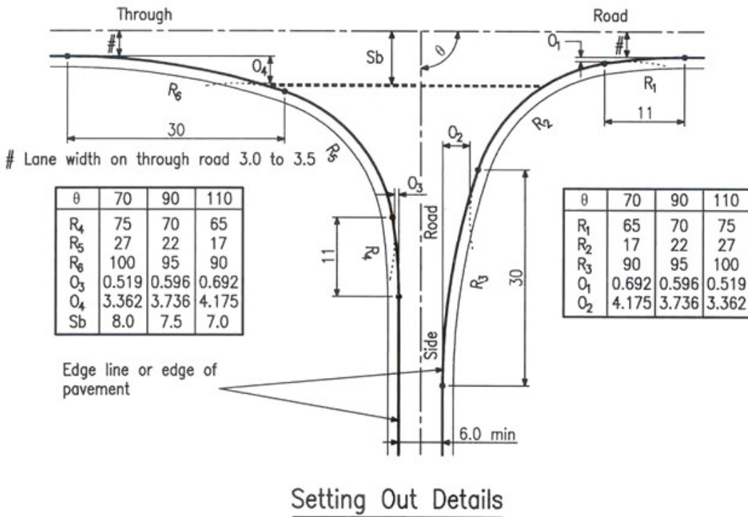
Figure D(b) – Details of type 'BAL' layout for rural sites to suit type 1 (double) road train operation
