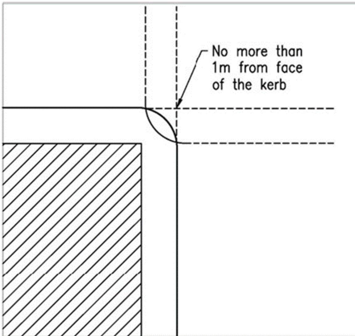
Figure 10.7(a) – Intersection of pedestrian crossings
